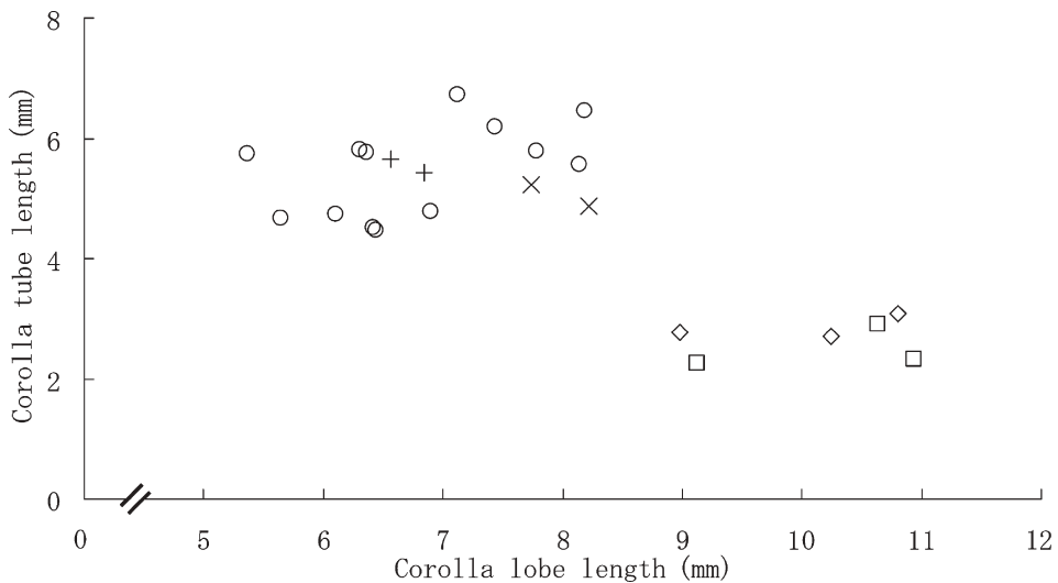
FIG. 3. Corolla tube and lobe lengths of plants investigated. \circ , Honshu (Japan); +, Shikoku (Japan); \times , Kyushu (Japan); \square , Iriomote (Ryukyus, Japan); \diamond , Taiwan.
